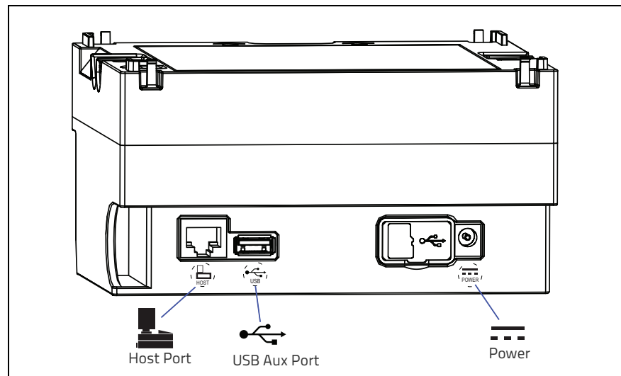
Figure 4. Scanner Features - Bottom View
