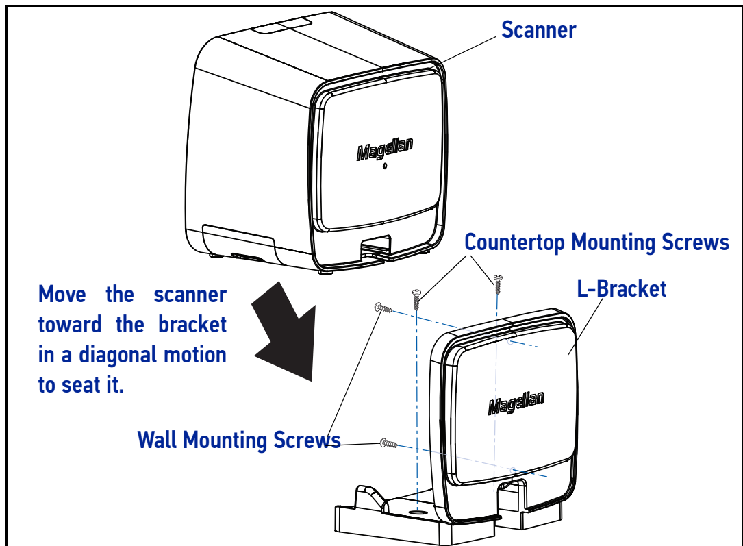
Figure 5. L-Bracket Mount
